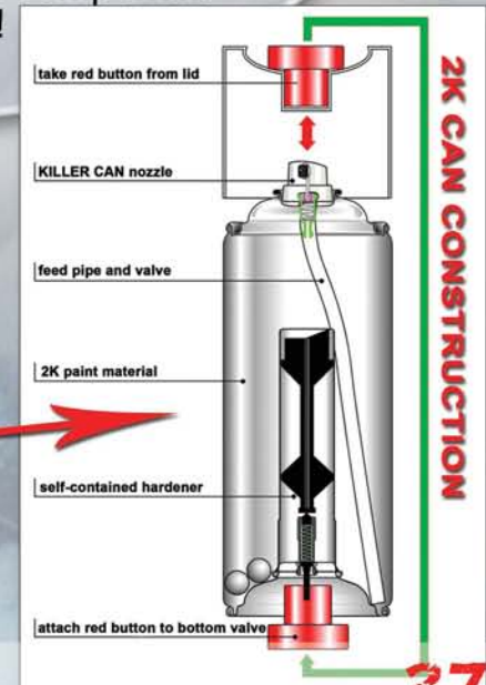
Internal view of a 2K can
